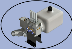
Hand pump with hydraulic switches (no electric power is required)
