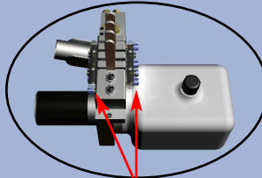
Optional HWH® AP43076 Leveleze® Indicator Light System Hand /electric pump with hydraulic switches
